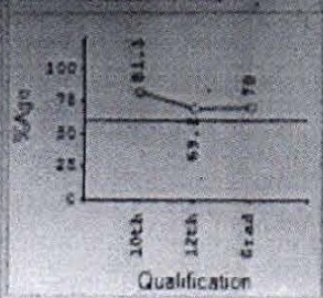
Academic Graph
