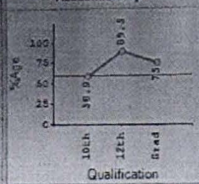
Academic Graph
