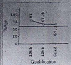
Academic Graph
